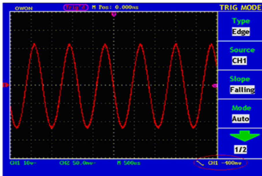
Fig.32 Wave Form Triggered on the Falling Edge
