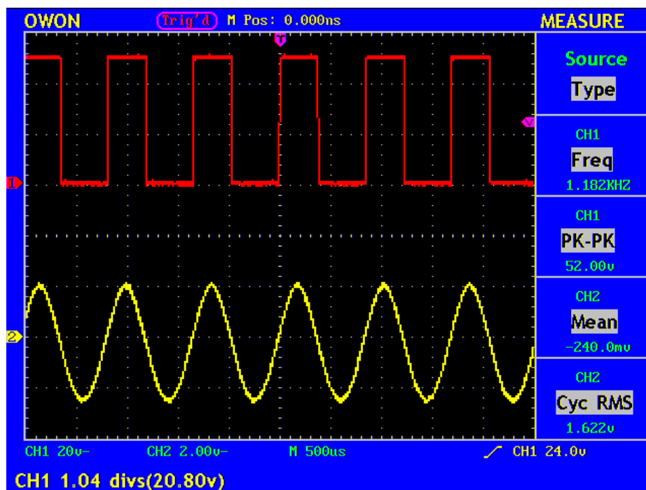
Fig.58 Automatic Measurement
