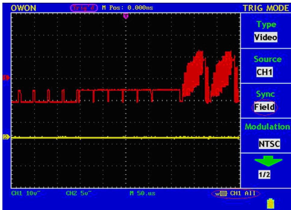
Fig.34 Wave Form Triggered in the Video Field
