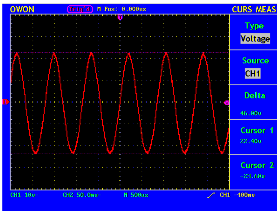
Fig.60 Wave Form of Voltage Cursor Measurement
