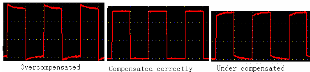
Fig.7 Displayed Waveforms of the Probe Compensation
