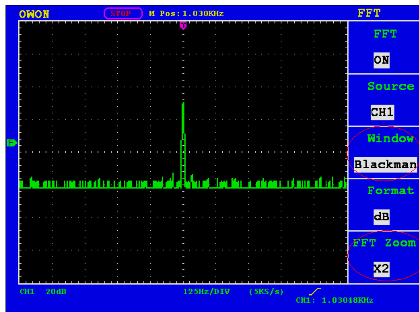
Fig.21 Blackman window
