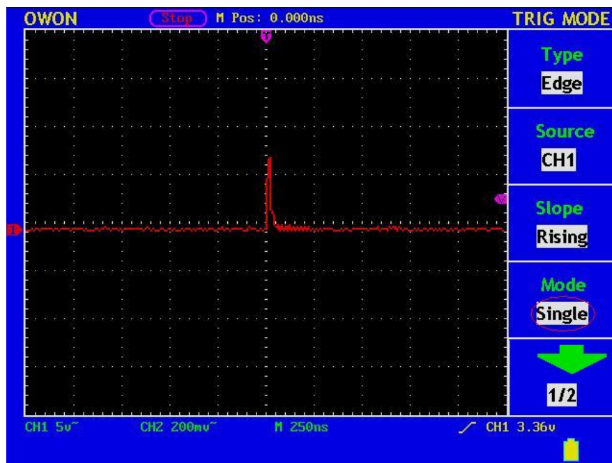
Fig. 66 Capture the Single Signal
