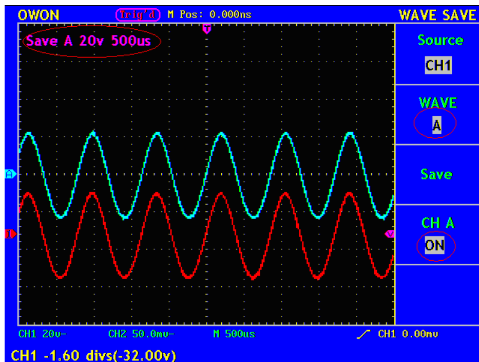
Fig.53 Wave Saving
