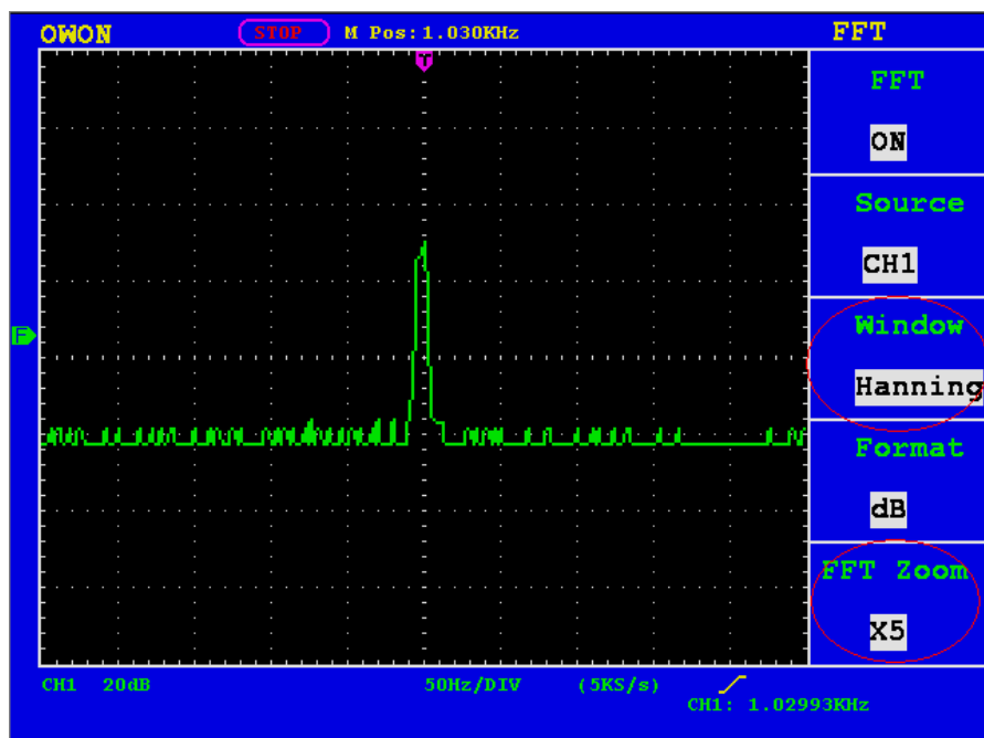
Fig.24 Hanning window
