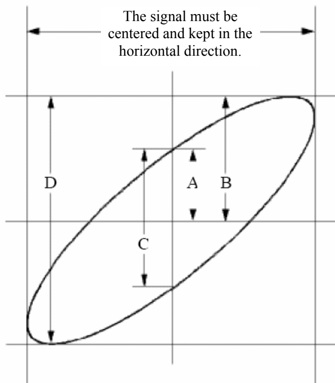
Fig.70 Lissajous Graph
