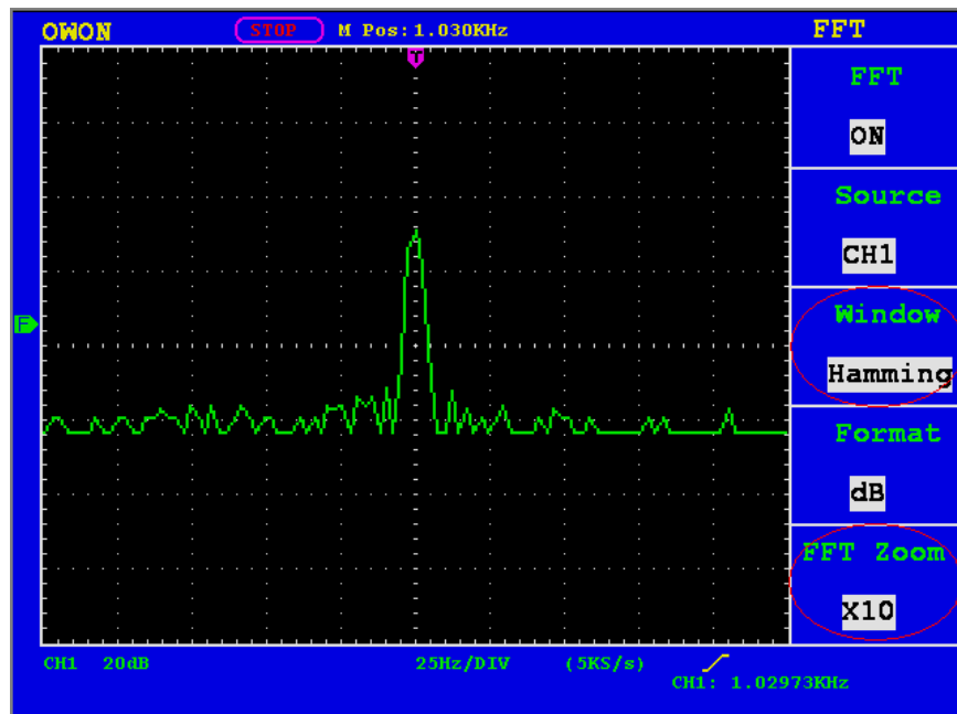
Fig.22 Hamming window
