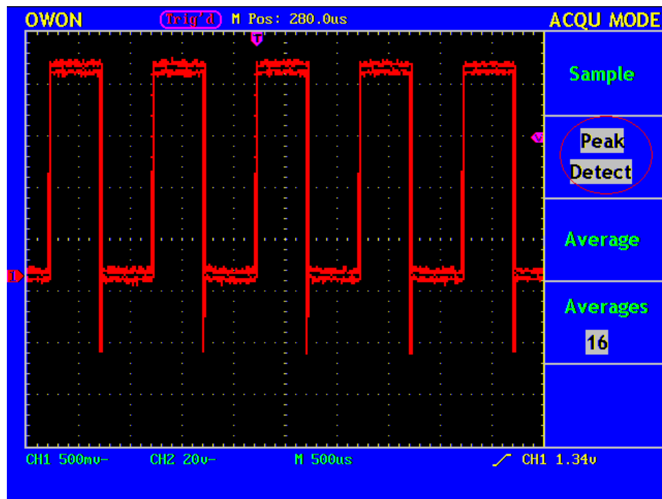
Fig.68 Wave Form of the Signal Containing Noises
