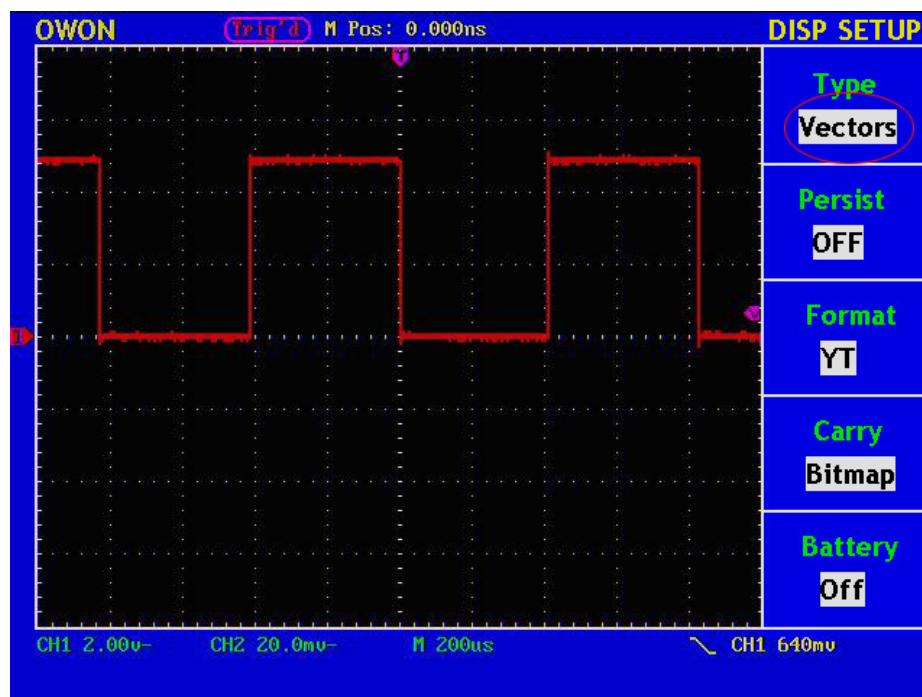
Fig.48 Display in the Vector Form
