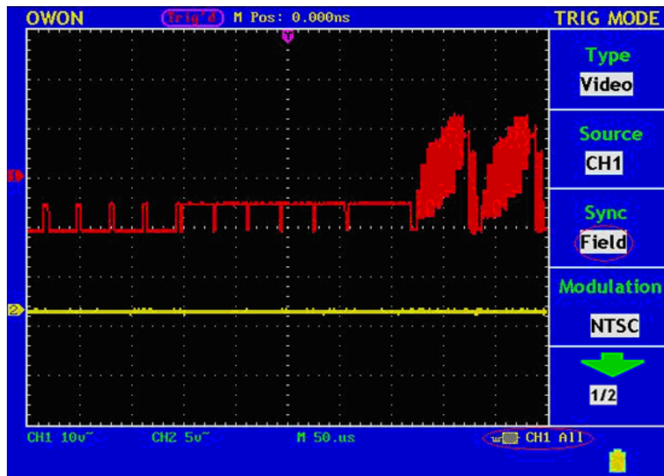
Fig. 71 Wave Form Obtained from Video Field Trigger
