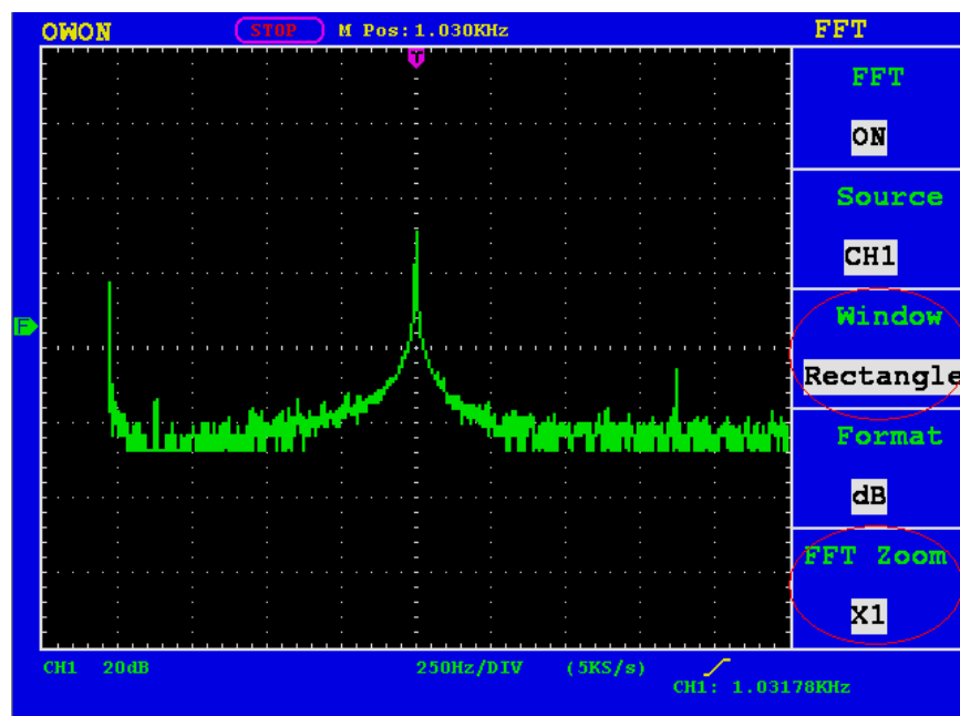
Fig.23 Rectangle window
